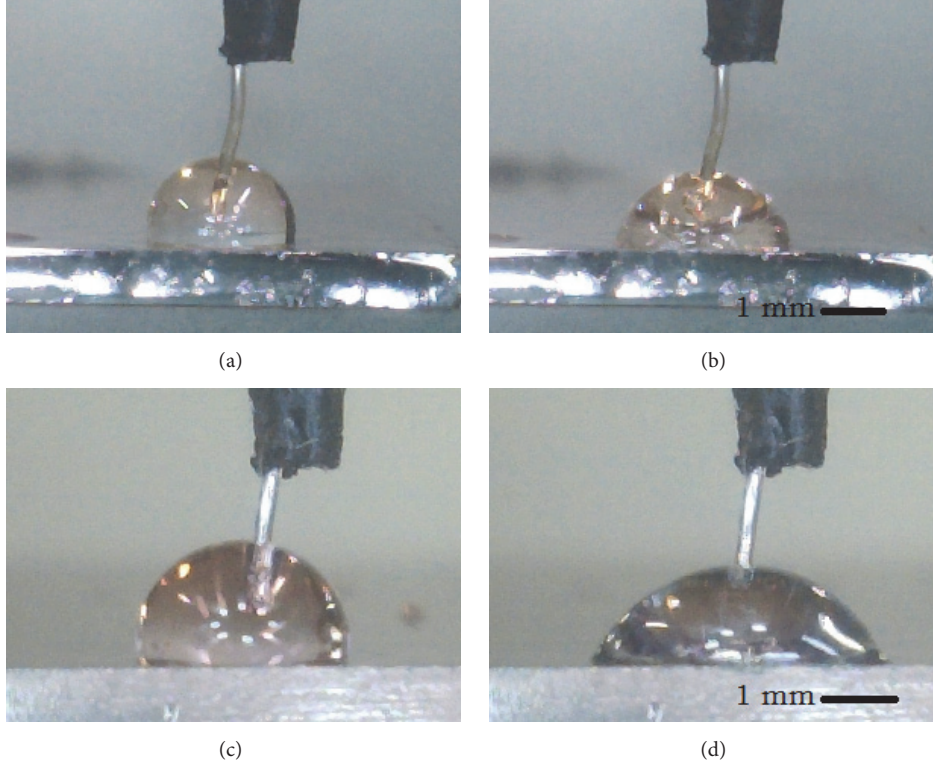
FIGURE 4: Change in droplet curvature and base diameter due to electrowetting actuation for deionized water: (a) at 0 V; (b) at 10 V. For a 0.5 \mu\text{m} nanofluid droplet, (c) a smaller contact angle at 0 V and (d) an enhanced electrowetting response at 10 V are observed.
